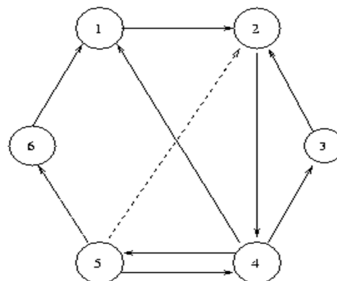
Gambar 29.5 Graph berarah
