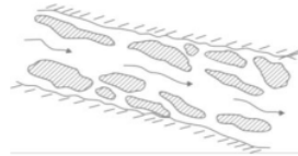
Figure 5. Dunes Shape Bars
