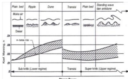
Figure 8. The Surface Form of Sediments Corresponds to The Type Of Flow That Flows On The Channel
