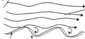
Figure 6. Erosion and Sediment Mechanisms
