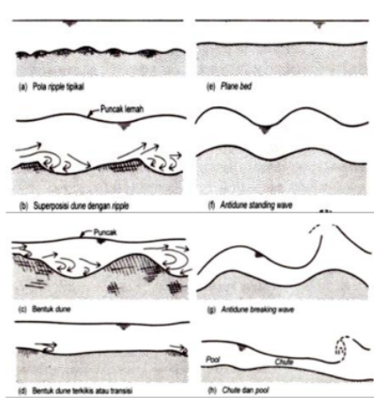
Figure 7. Form of Sediment Stacking on Channel Basis
