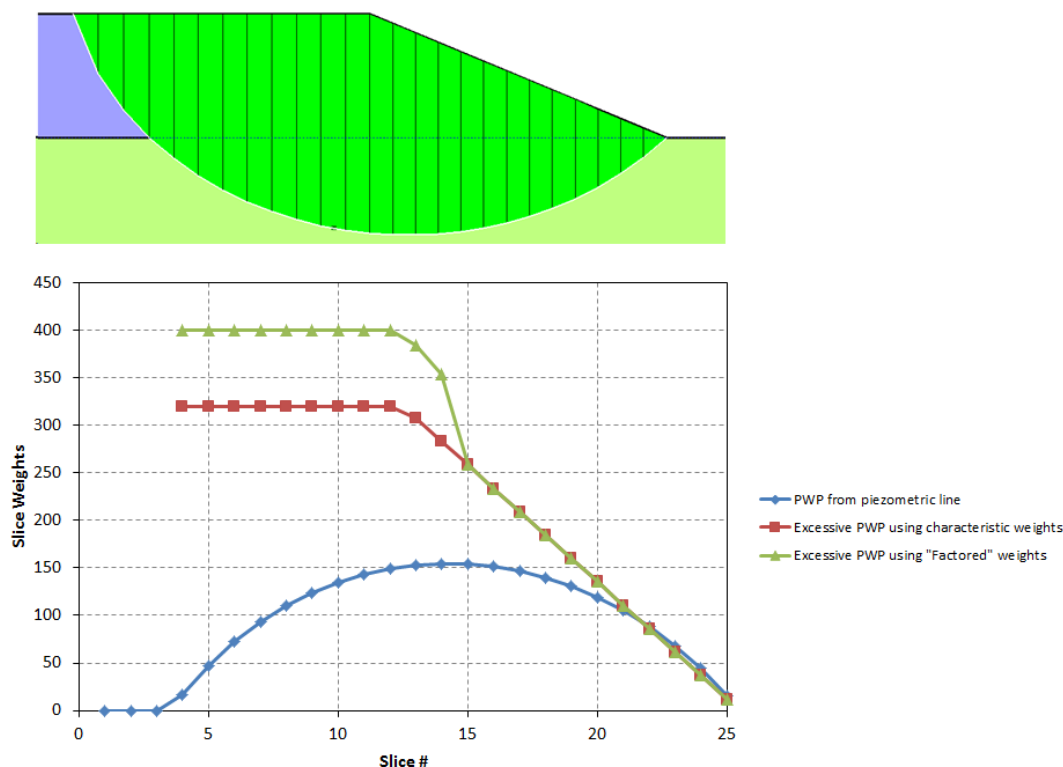
Figure 12-3 Excess pore-water pressures resulting from applying a partial factor to the unit weight of unfavorable slices
