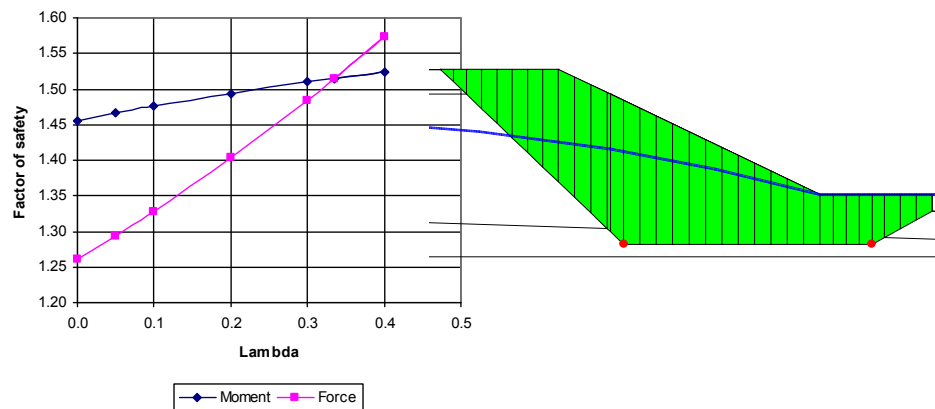
Figure 2-7 Typical situation for a block slip surface
