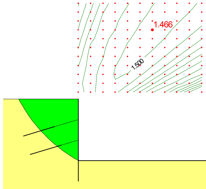
Figure 9-29 Stability analysis based on finite element stresses
