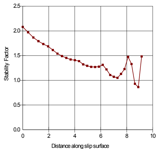
Figure 9-27 Local safety factors along the slip surface
