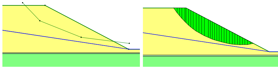
Figure 4-35 Fully specified slip surface (Left) after optimization (Right)
