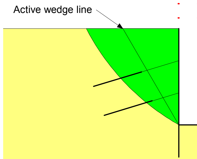
Figure 9-31 Position of critical slip surface relative to active wedge
