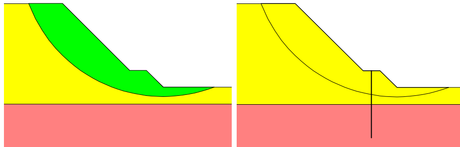
Figure 9-34 Finite element analysis with a shear wall
