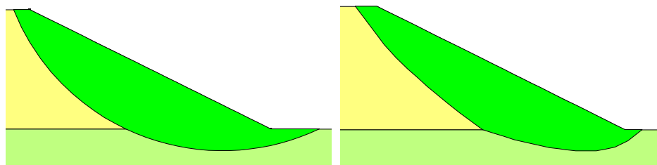
Figure 4-30 Traditional (Left) and Optimized (Right) slip surface
