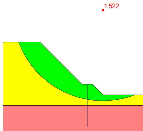
Figure 9-35 Factor of safety with the shear wall in place
