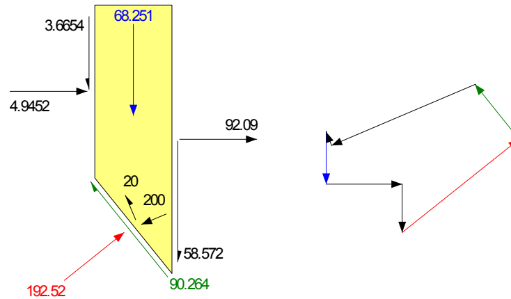
Figure 9-12 Slice free body with a shear force
