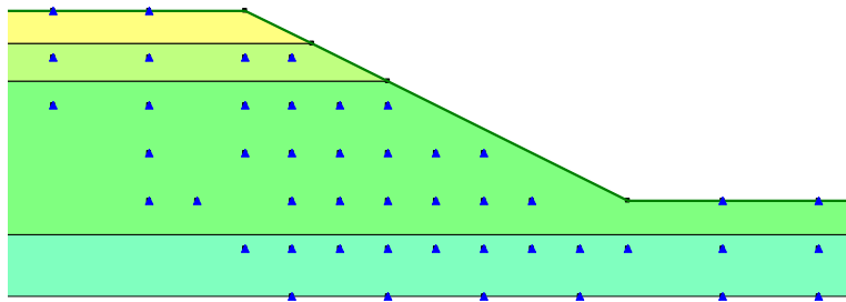
Figure 8-5 Grid of pore water pressure head
