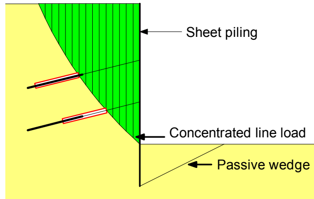
Figure 9-20 Embedded sheet pile
