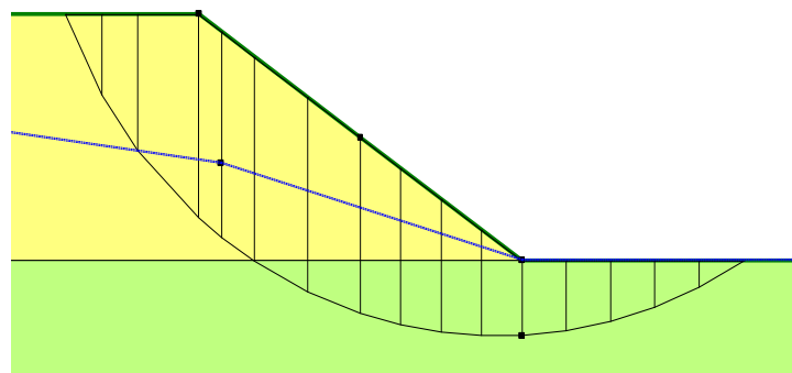
Figure 5-8 Discretization when the specified number is 15 slices
