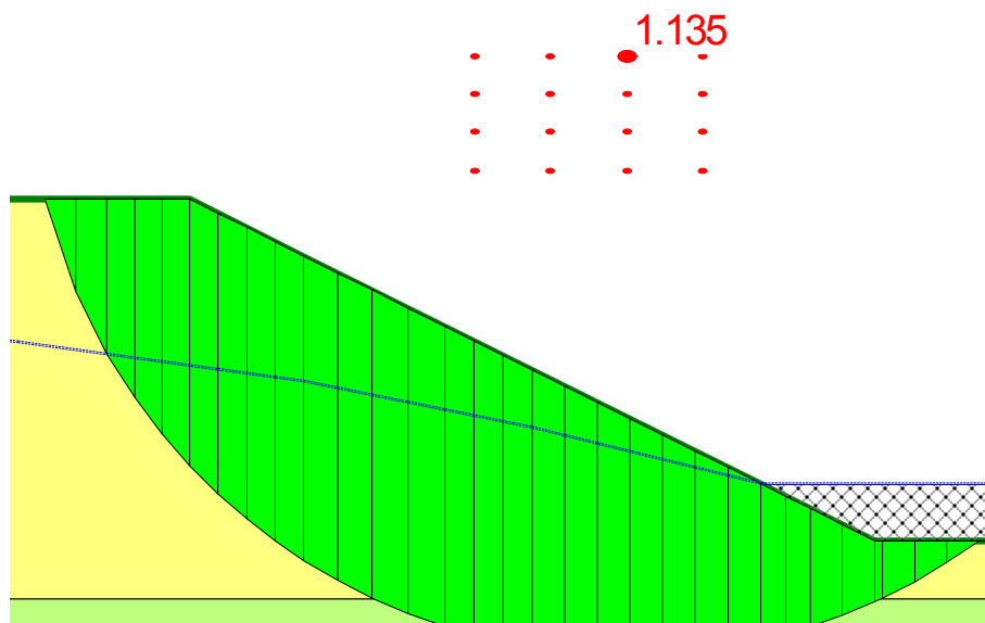
Figure 3-22 Corps of Engineers assumption #2
