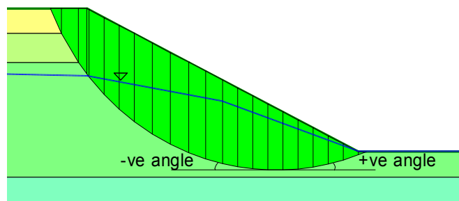
Figure 7-8 Sign convention of inclination angle used in SLOPE/W
