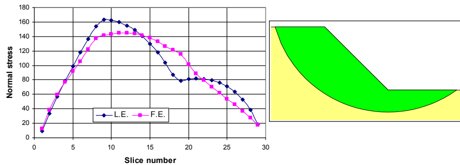
Figure 3-34 Normal stress distribution along a deep slip surface
