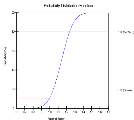
Figure 11-14 Factor of safety probability of failure
