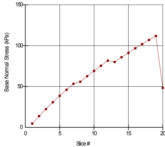
Figure 9-7 Stress distribution along slip surface when reinforcement load is distributed
