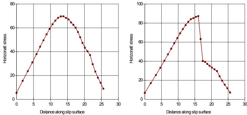
Figure 9-36 Horizontal stresses along slip surface without and with pile
