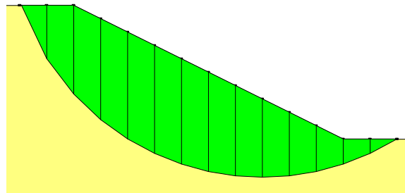
Figure 3-4 Case for hand-calculations
