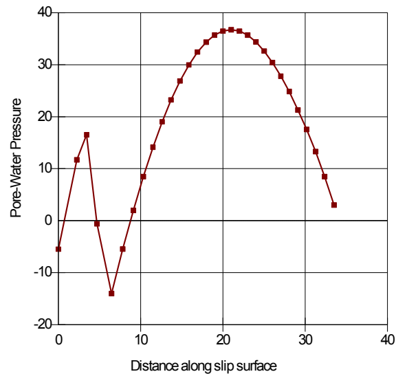
Figure 8-8 Pore-water pressure distribution along slip surface
