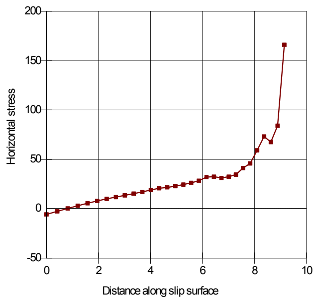
Figure 9-26 Horizontal stress along slip surface
