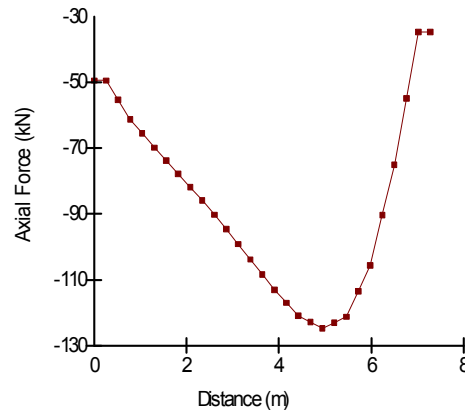
Figure 9-24 Axial force in nail
