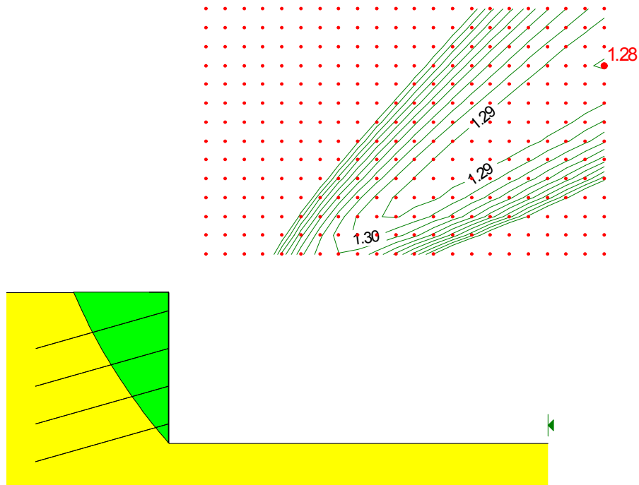
Figure 9-23 SLOPE/W stability analysis results based on SIGMA/W stresses
