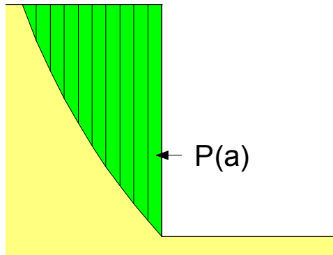
Figure 9-33 Active earth pressure calculation
