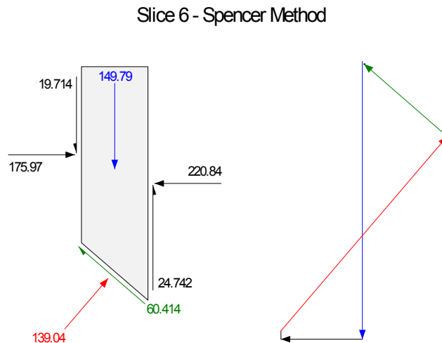
Figure 3-14 Free body diagram and force polygon for the Spencer method
