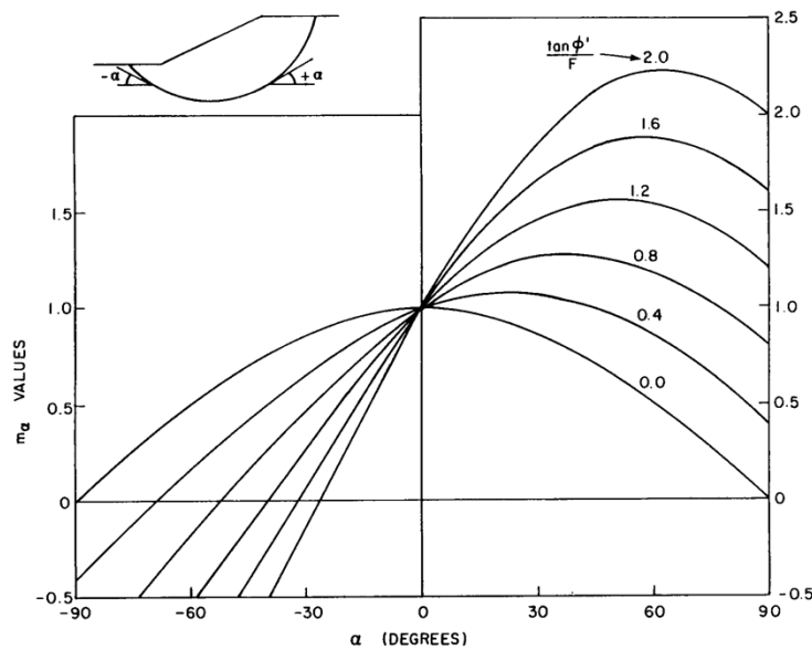
Figure 14-4 Magnitude of m_\alpha for various \alpha , \phi , and F values
