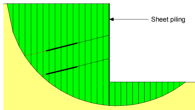
Figure 9-21 Deep seated failure
