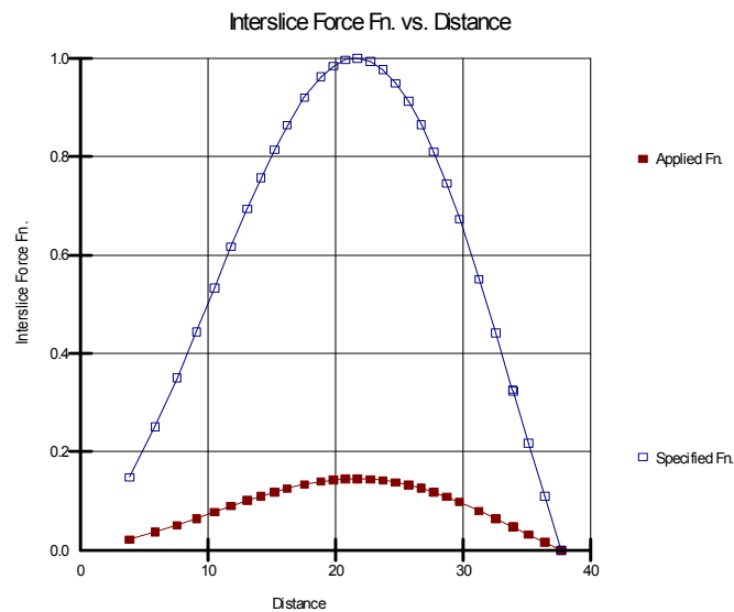
Figure 3-17 Interslice half-sine functions
