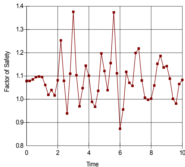
Figure 3-37 Factors of safety variations during earthquake shaking
