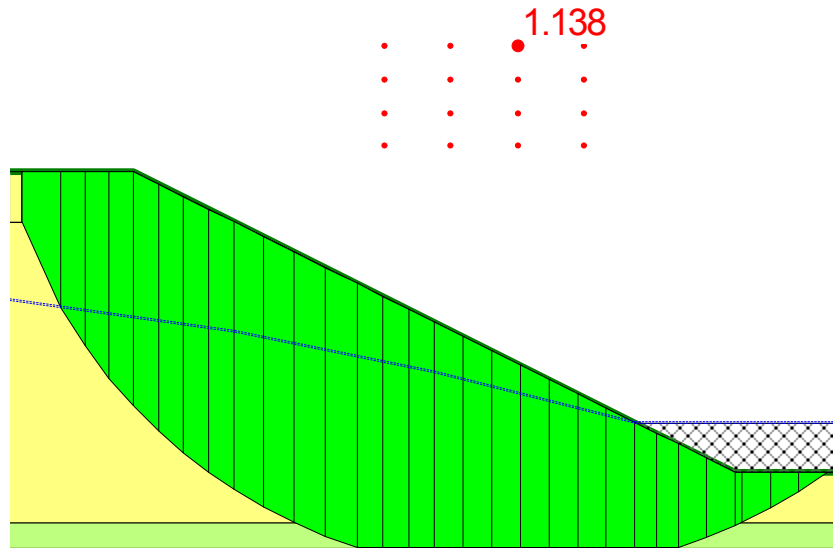
Figure 3-25 Lowe-Karafiath safety factor
