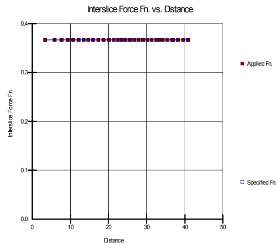
Figure 3-20 Corps of Engineers #1 interslice function
