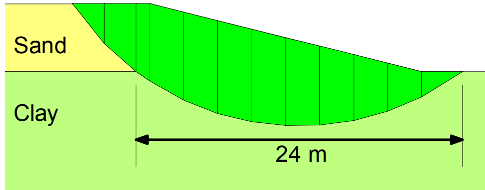
Figure 11-16 Case with statistical variability in the clay
