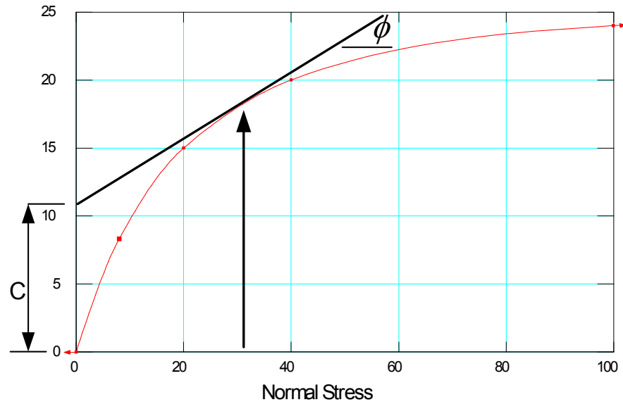
Figure 7-6 General data-point shear-normal function
