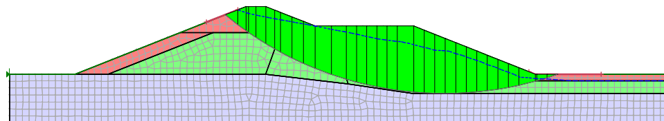
Figure 10-19 A slip surface passing some liquefied elements
