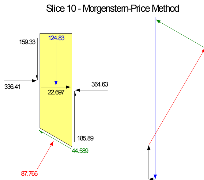
Figure 10-5 Slice forces with a k_v specified
