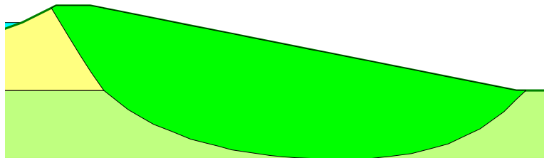
Figure 4-33 Slip surface when Block method optimized
