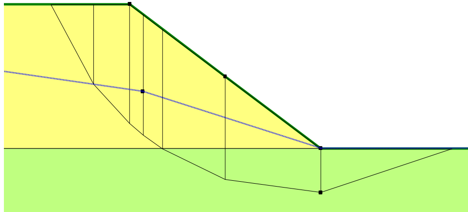
Figure 5-7 Sections in the slice discretization process
