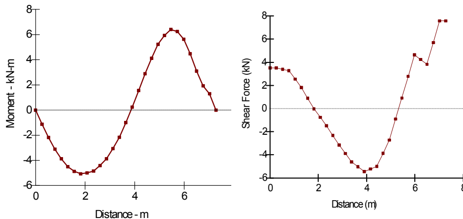
Figure 9-25 Moment and shear distribution in the nail
