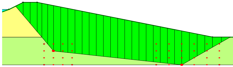
Figure 4-32 Slip surface when using the Block method
