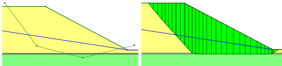
Figure 4-34 Fully specified slip surface (Left) after optimization (Right)
