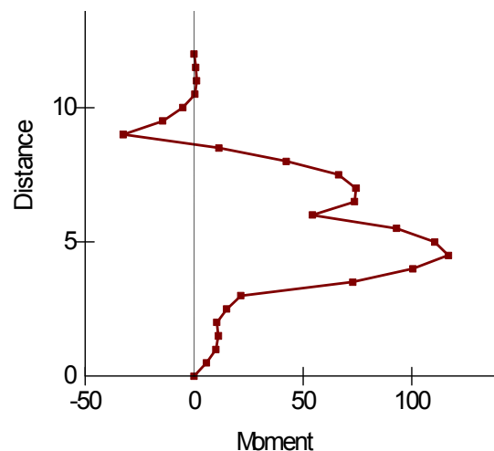
Figure 9-32 Moment distribution in sheet piling
