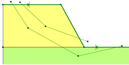
Figure 4-51 Slip surface enter and exit beyond the limits
