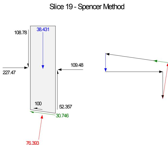
Figure 9-19 Shear force of pile on slice free body
