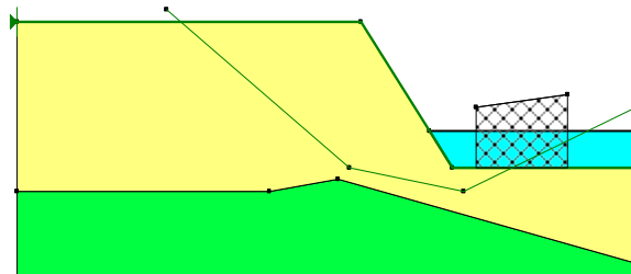
Figure 4-46 Slip surface intersecting a pressure line inside a zero strength material
