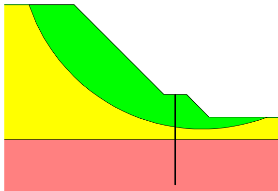
Figure 9-18 Slope reinforced with a pile or dowel
