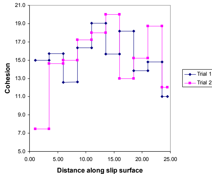
Figure 11-19 Strength variation along the slip surface when soil is sampled for every slice
