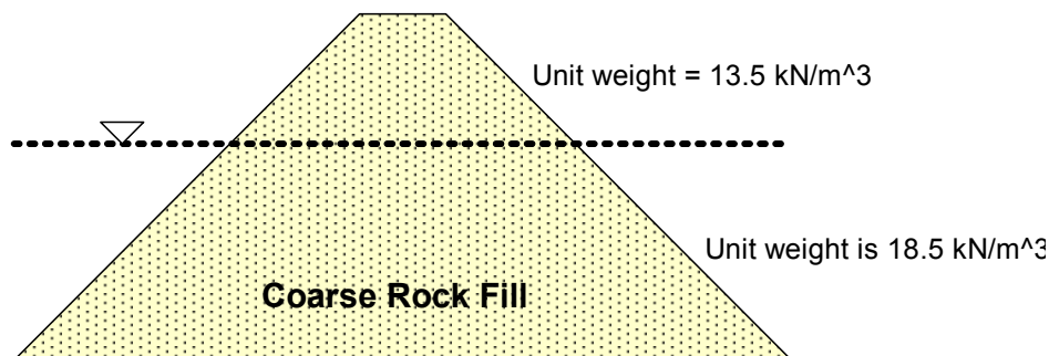
Figure 7-14 Different unit weight above and below the water in rock fill
