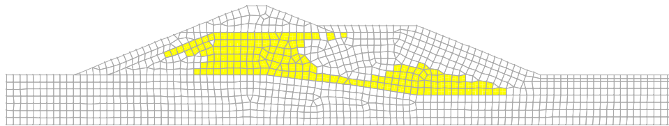
Figure 10-18 Example QUAKE/W analysis showing some liquefied elements
