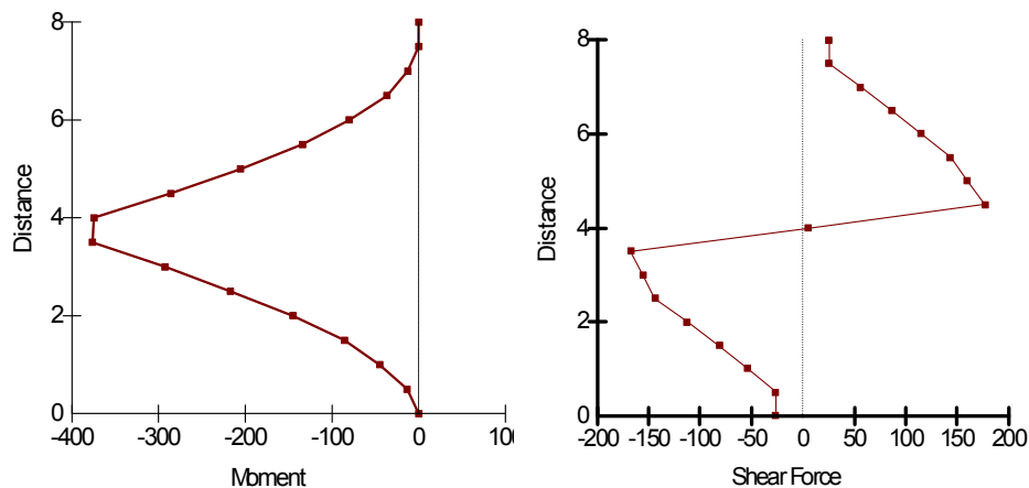
Figure 9-37 Moment and shear distribution in wall
