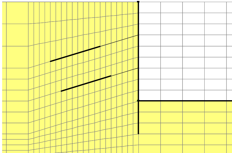
Figure 9-28 A sheet pile wall with pre-stressed tie-back anchors
