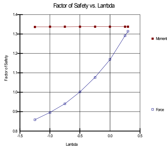
Figure 4-49 No intersecting point in a GLE formulation
