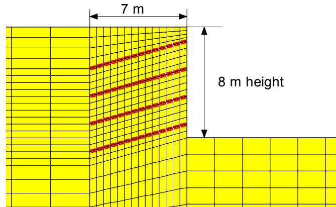
Figure 9-22 A vertical wall retained with nails
