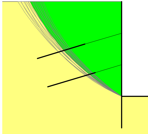
Figure 9-30 Twenty most critical slip surfaces
