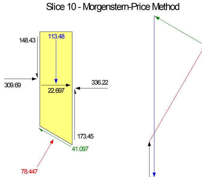
Figure 10-4 Horizontal seismic inertial force at slice centroid
