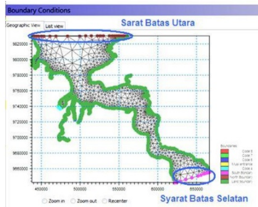
Gambar 4. Boundary Condition
