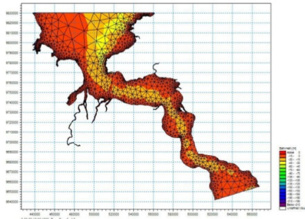
Gambar 3. Mesh Grid Model
