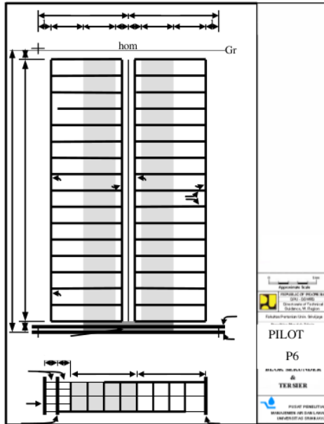
Gambar 5. Lay out blok sekunder dan blok tersier di Telang I (Land and Water Management Research Centre, 2004); (Sartika, 2009)
