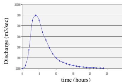
Fig 3. The unit hydrograph Synthetic of Sekanak sub-basin
