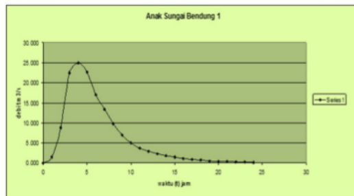
Fig 5. Synthetic hydrograph unit of Bendung watershed
