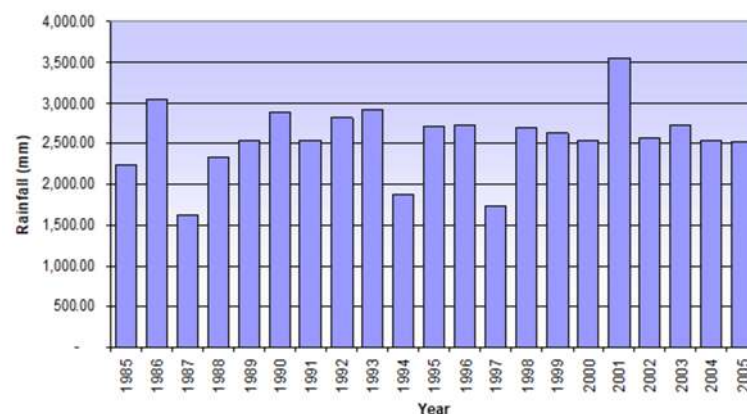
Figure 4. Annual rainfall telang I from 1985-2005 (Kenten rainfall station, 2008); (Sartika, 2009)
