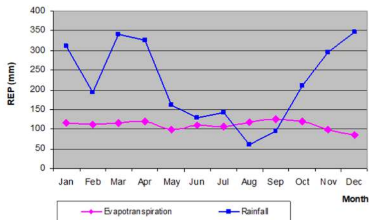
Figure 5. Montly rainfall and potential evapo-transpiration of telang I from 1996- 2005 (Kenten rainfall station, 2008); (Sartika, 2009)
