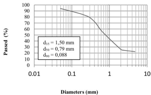
Fig. 7. Grain size distribution in SPD canal
