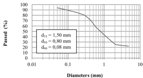
Fig. 8. Grain size distribution in SDU canal
