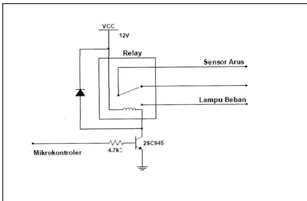
Gambar 4. Rangkaian Relay
