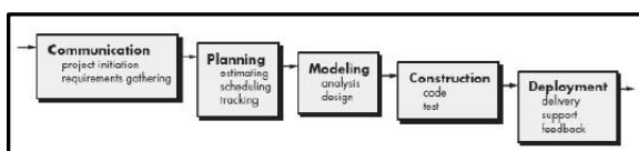
Gambar 1. Tahapan model Waterfall
