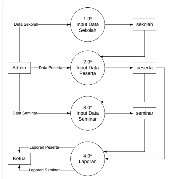
Gambar 3. DFD Level 0
