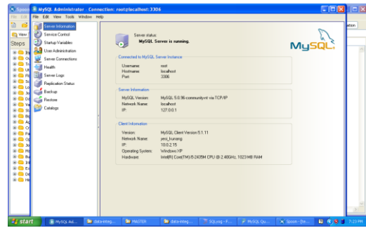
Gambar 3. Proses extract
