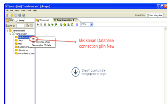
Gambar 1. data connection
