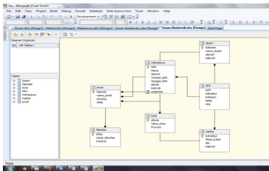
Gambar 6. Star schema
