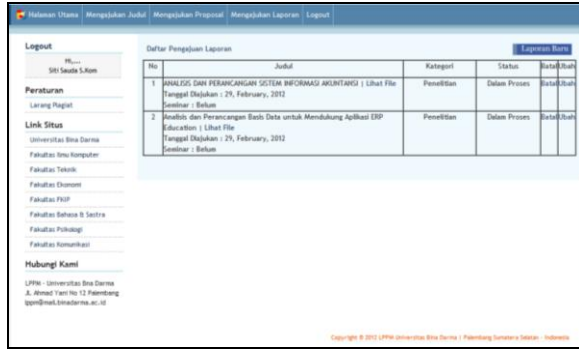
Figure 17 Report Page
