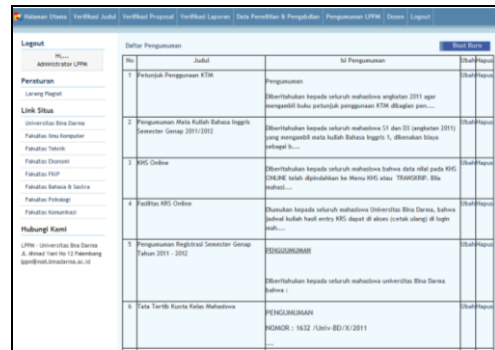
Figure 31 Announcements LPPM
