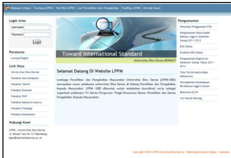
Figure 4 Home Menu
