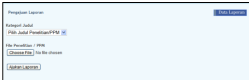
Figure 18 Report Form
