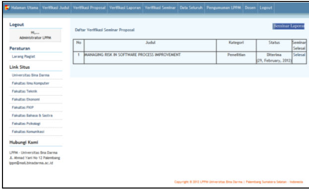
Figure 28 conference verification
