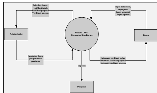
Figure 3 context diagram
