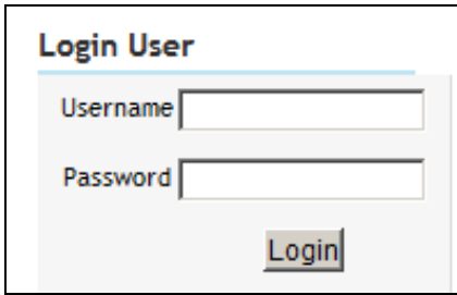
Figure 10 Login User
