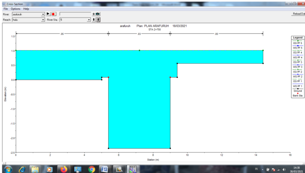
Fig. 7. The pattern of water flow movement in the Buah river Sta.2+750
