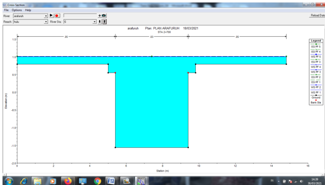
Fig. 8. The pattern of water flow movement in the Buah river Sta.2+700
