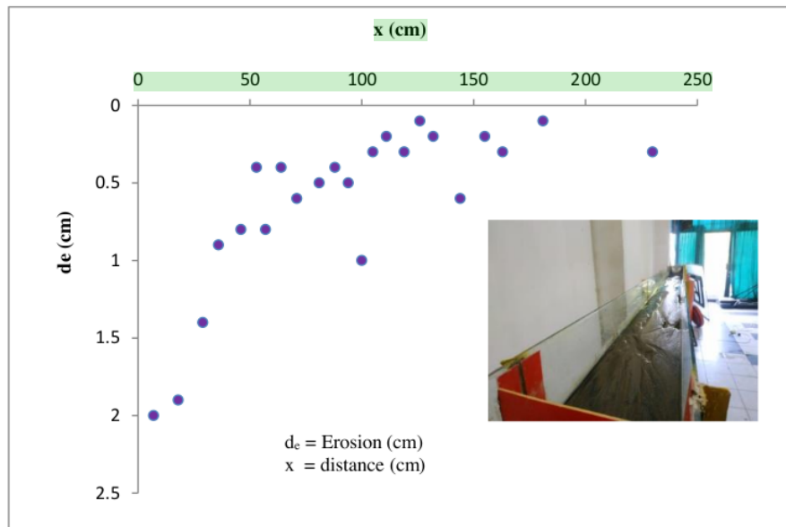
Fig. 7. Plotting The Results of the erosion depth (de) during the "running test" for 30 minutes
