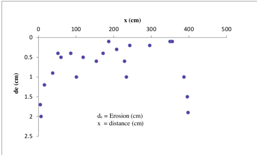
Fig. 3. Plotting The Results of the erosion depth (de) during the "running test" for 10 minutes
