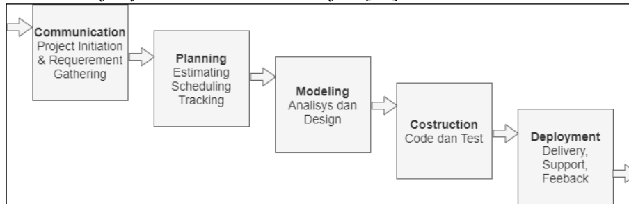
Gambar 1. Model waterfall
