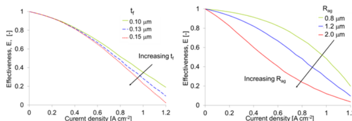
Figure 4: The catalyst effectiveness as a function of current density for various values of the thin film thickness (with t_f = 0.1, 0.13 and 0.15 \mu m ) and the agglomerate radius (with R_{ag} = 0.8, 1.2 and 2.0 \mu m )
