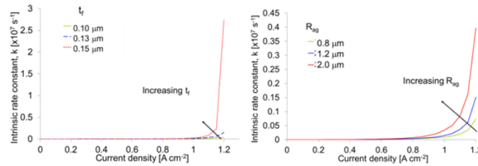
Figure 2: Intrinsic rate constant as a function of current density for various values of the thin film thickness (with t_f = 0.1, 0.13 and 0.15 \text{ }\mu\text{m} ) and the agglomerate radius (with R_{ag} = 0.8, 1.2 and 2.0 \text{ }\mu\text{m} )
