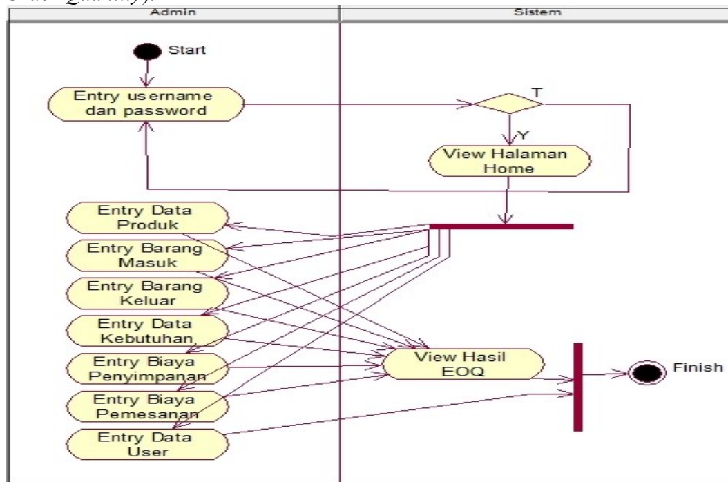
Gambar 4.4 Activity Diagram Admin
