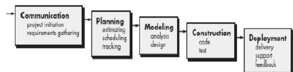
Gambar 1. Waterfall Pressman
