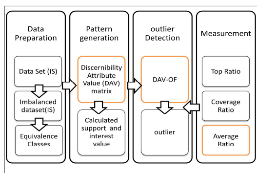
Figure 4: The proposed outlier detection modelling process
