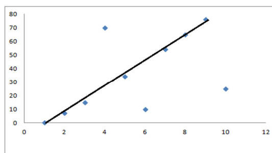
Figure 1: Outliers are indicated by the points far from the distribution of data
