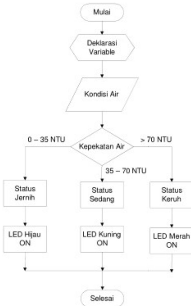
Gambar 6 Flowchart Rangkaian
