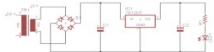
Gambar 5 Rangkaian Power Supply Regulator
