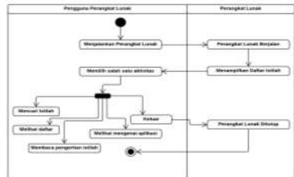
Gambar 4. Activity Diagram
