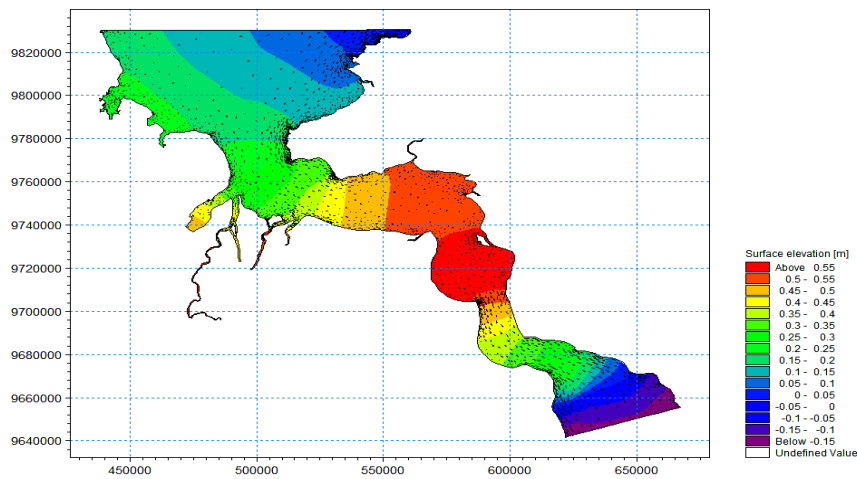
Fig. 3. Model hydrodynamic surface elevation Watersheds [5]
