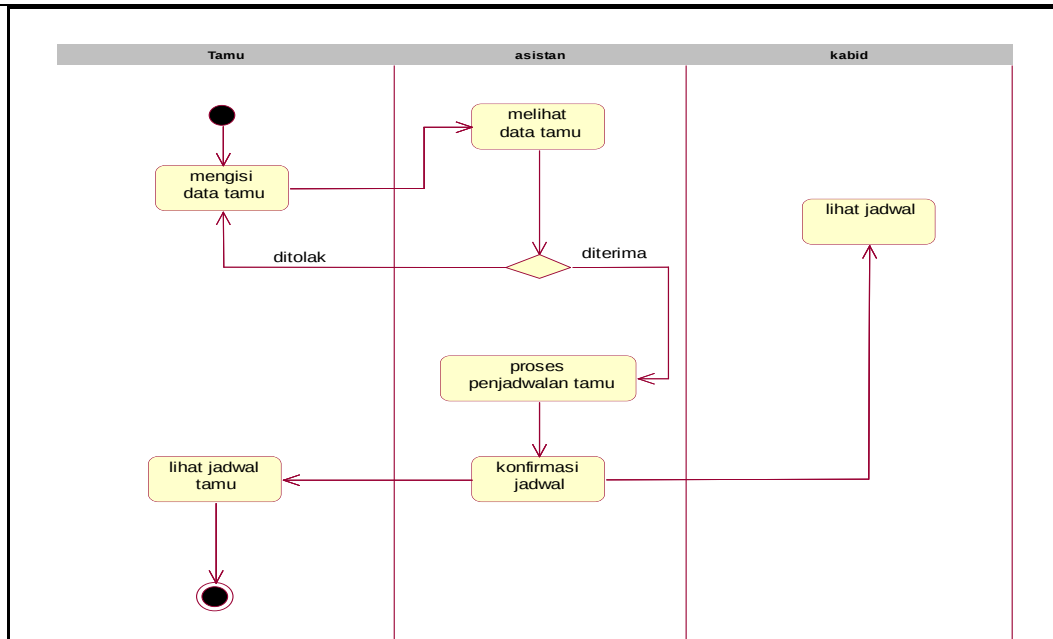
Gambar 3. Activity Diagram
