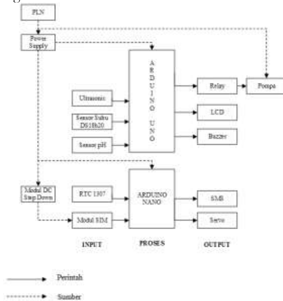
Gambar 1 Blok Diagram
