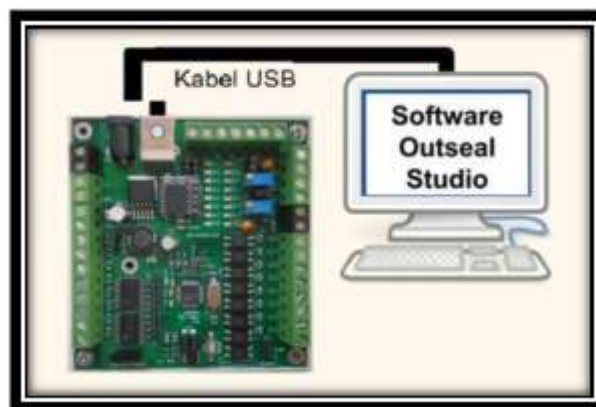
Gambar 3. Outseal PLC
