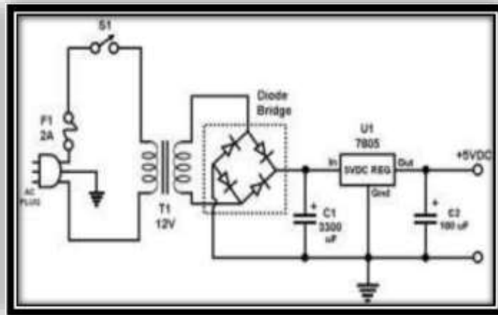
Gambar 7. Catu daya 5V DC
