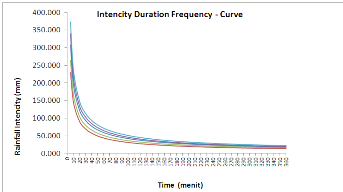
Figure 1. IDF (Intensity Duration Frequency) Curve
