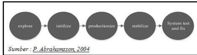
Gambar 1.1 Metode Mobile-D
