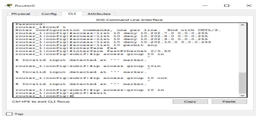
Gambar 5. Access List
