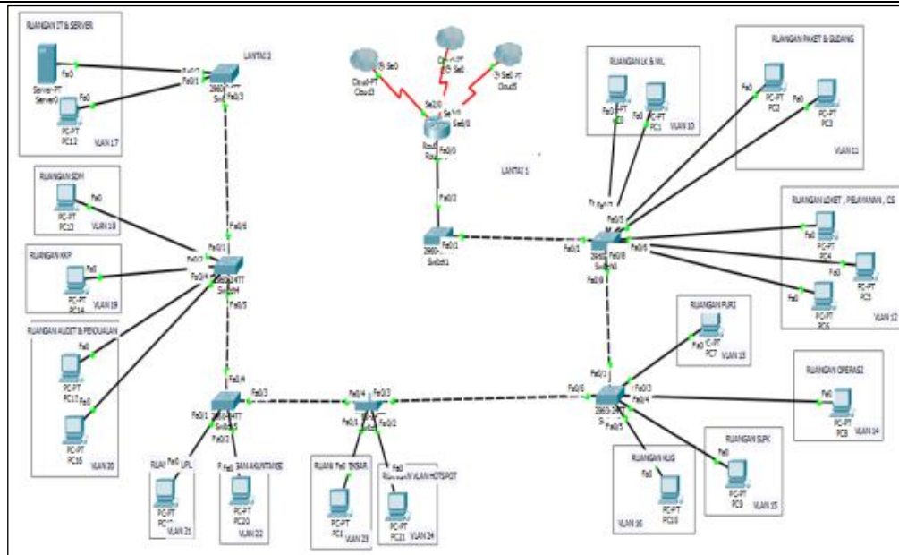
Gambar 3. Topologi logis disertakan vlan
