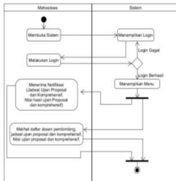
Gambar 3 Activity Diagram Mahasiswa
