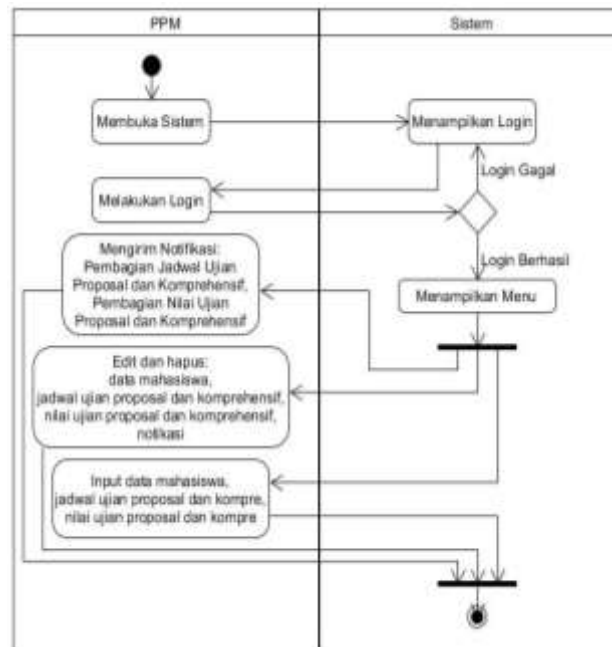
Gambar 4 Activity diagram PPM
