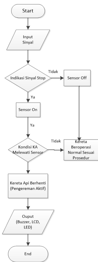
Gambar 6 Flowchart Rangkaian
