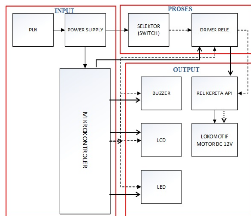
Gambar 5 Blok Diagram Rancang Bangun sistem Pengereman Emergency
