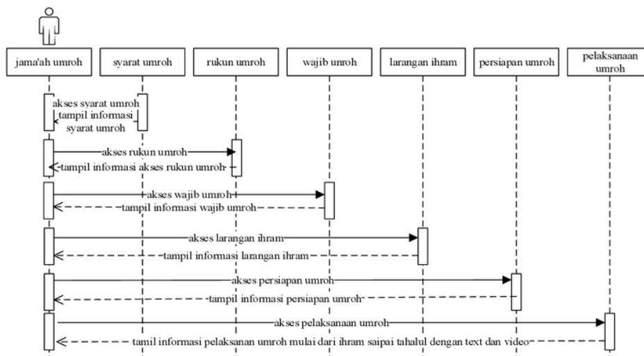
Gambar 4. Sequence Diagram
