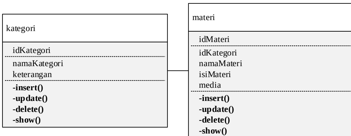
Gambar 2. Class diagram
