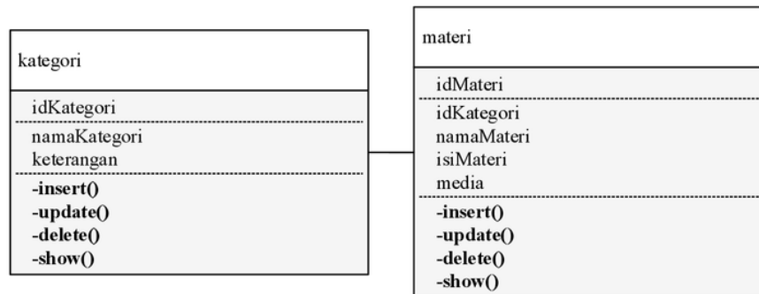
Gambar 2. Class Diagram
