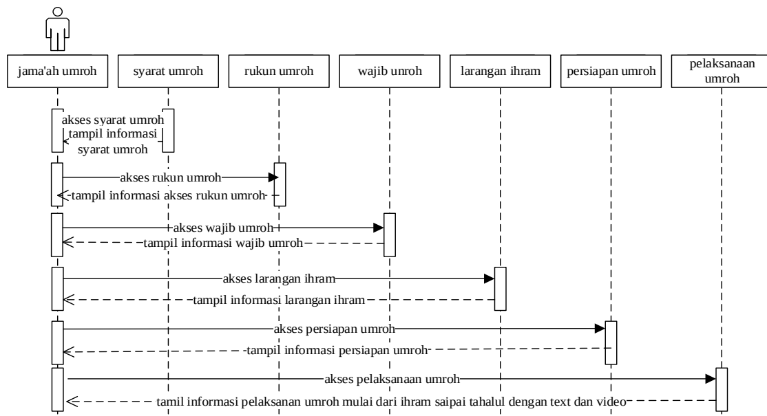
Gambar 4. Sequence diagram
