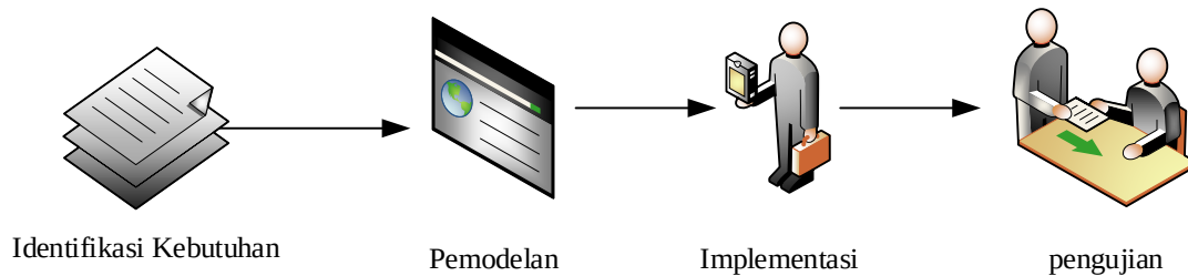
Gambar 1. Proses penelitian
