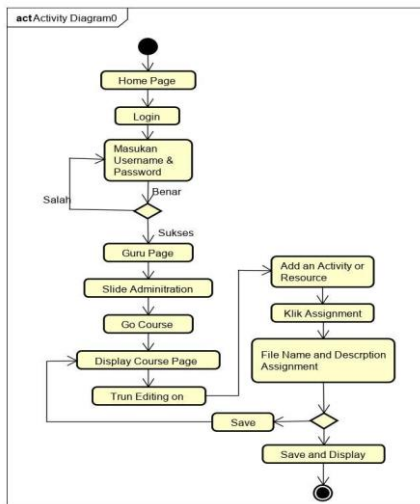
Gambar 4 Activity diagram Add Assignment
