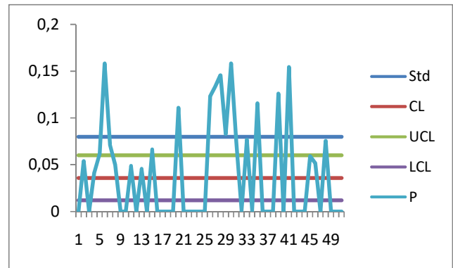
Gambar 2. Peta kendali Control Cacat C 100% Inspection
