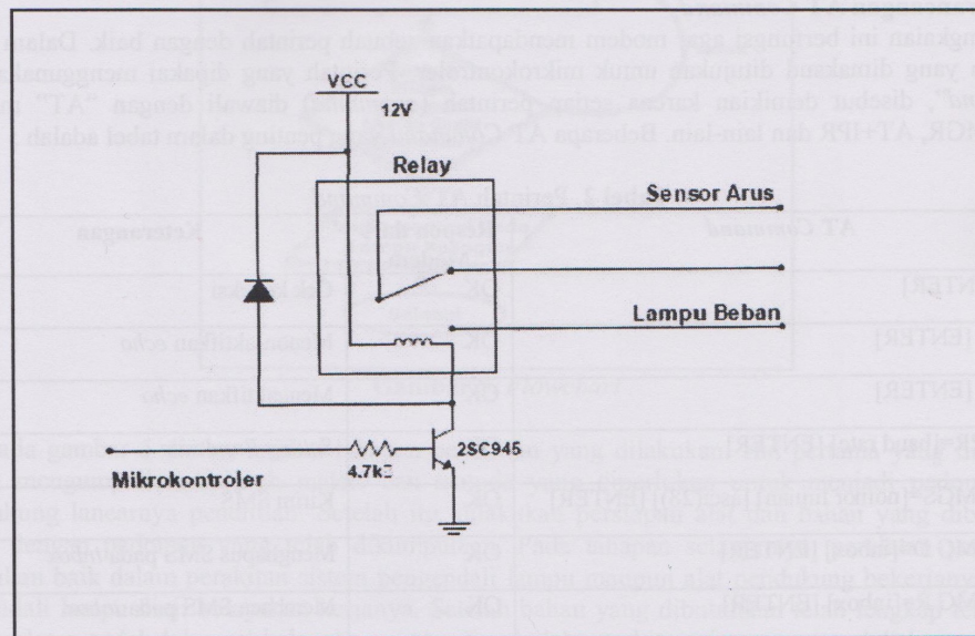
Gambar 4. Rangkaian Relay
