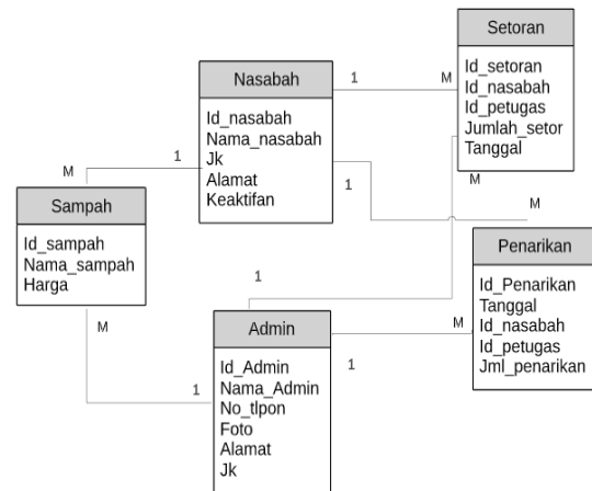
Figure 3. Entity Relationship Diagram
