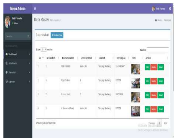
Figure 4. Member data
