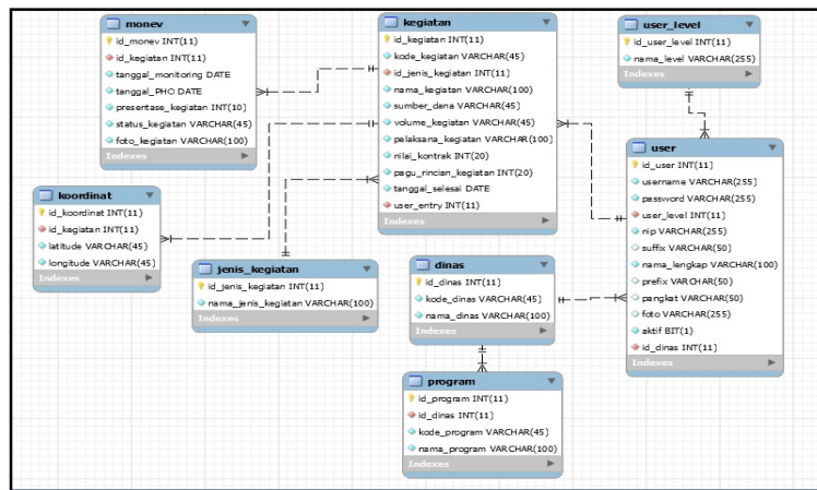
Gambar 3. Class Diagram
