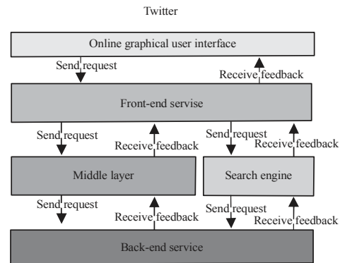
Fig. 2: Architecture of Twitter
