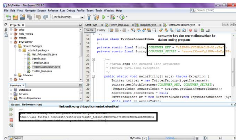
Fig. 4: Code PIN authentication
