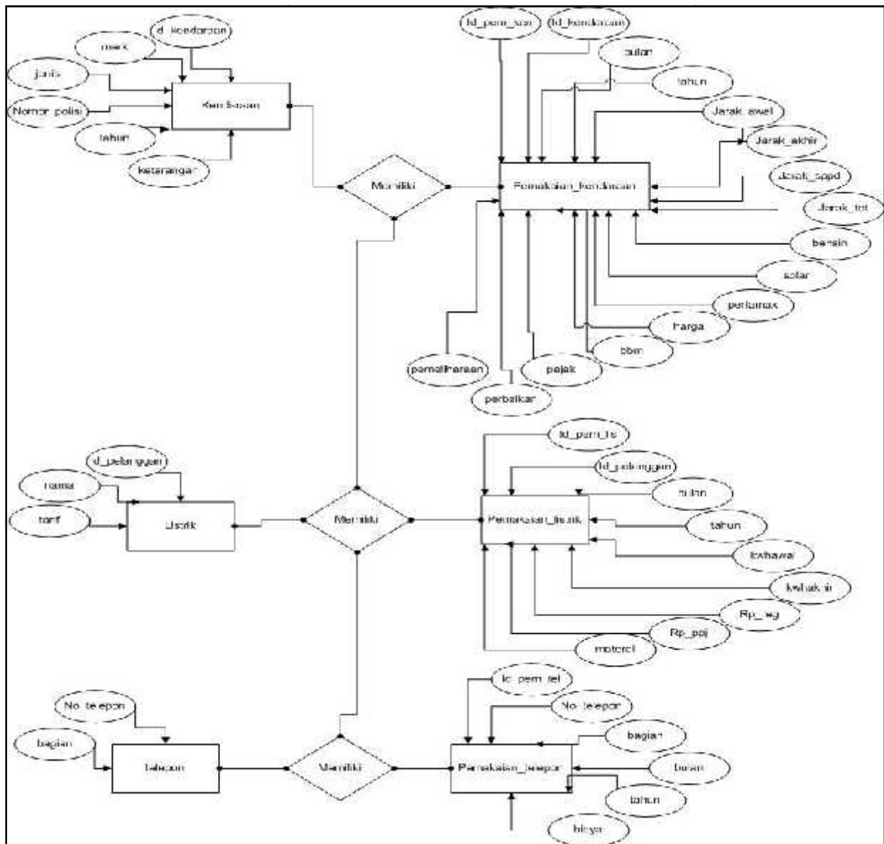
Gambar 4. Entity Relationship Diagram (ERD)
