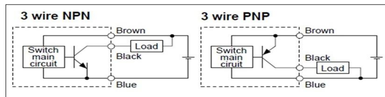
Gambar 5. Diagram wiring sensor aliran air
